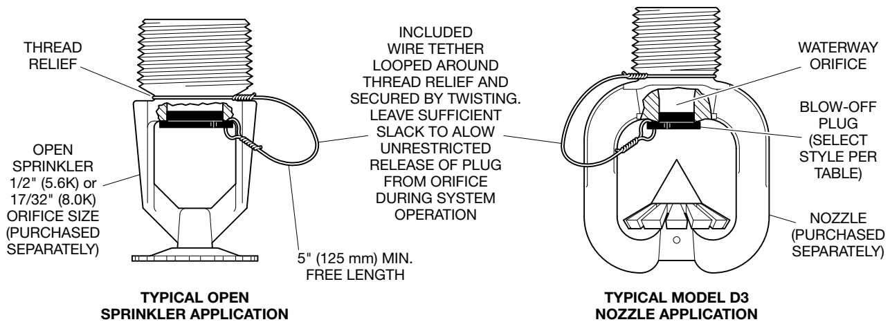
FIGURE 1 BLOW-OFF PLUGS
