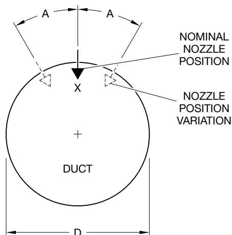
FIGURE 4 NOZZLE HYDRAULIC REQUIREMENTS AND POSITION VARIATION
