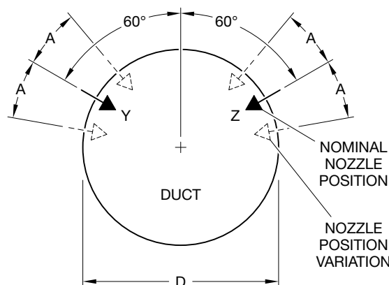
FIGURE 4 NOZZLE HYDRAULIC REQUIREMENTS AND POSITION VARIATION
